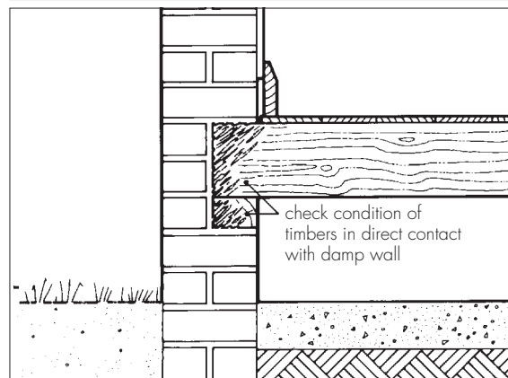
Figure 2 Check embedded timber for decay
